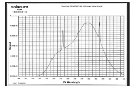
UV-Pontoon Spectral Power Distribution Covers 280-380 nm
