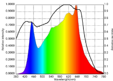
Impact Series Model 151-740 Spectral Power Distribution Covers 400-700nm against McCree
